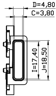
SECTION B-B
